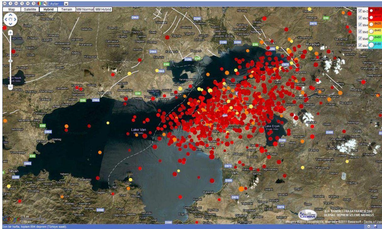
Distribution of aftershock sequences as of 27 October 2011 09:00 local time.
