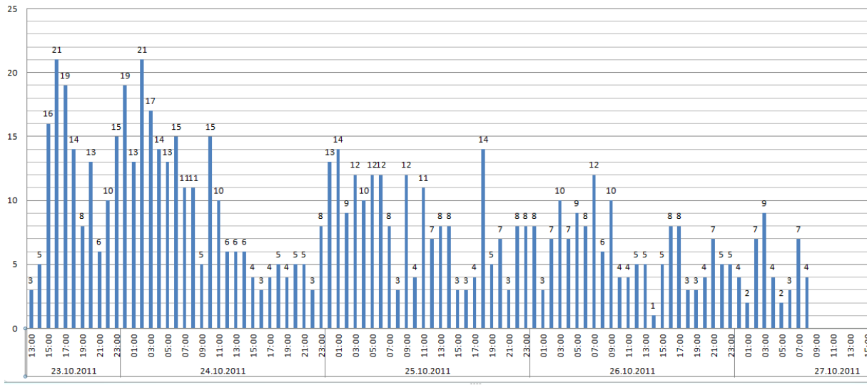
The figure above shows the hourly distribution of number of aftershock occurrences.
